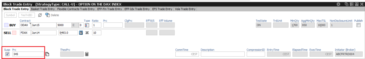
Fig. 86: Screenshot of the TES - Block Trade Entry view showing the entry of a suspended block trade
