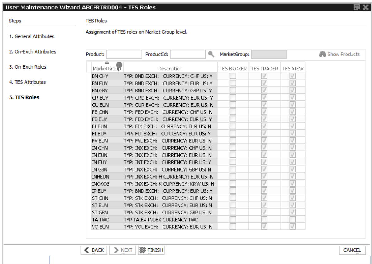
Fig. 158: Screenshot of the User Maintenance Wizard showing the TES Roles tab
