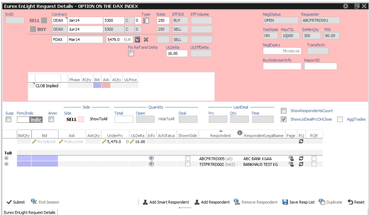
Fig. 104: Screenshot of the Eurex EnLight Request Details for a Vola strategy when UL and Delta should be negotiated
